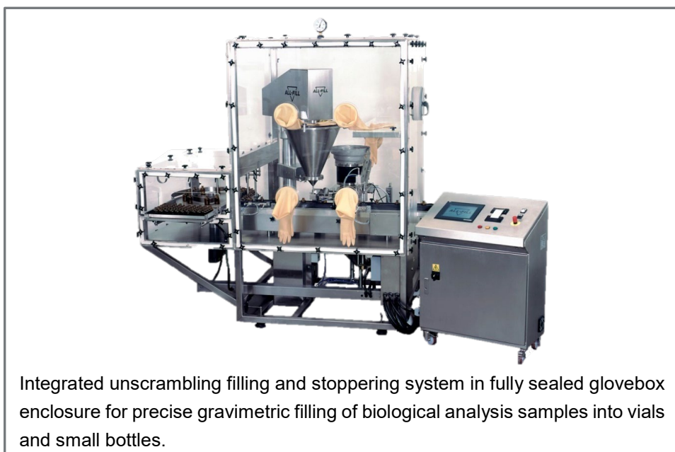
Series 1 Micro-Fill unit for laboratory and production use. 10mg to 50g. Inclusive of servo drive, colour touch-screen HMI and integral workstation.
